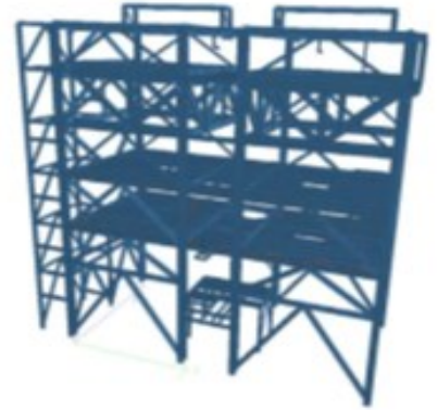
● Process Structure
