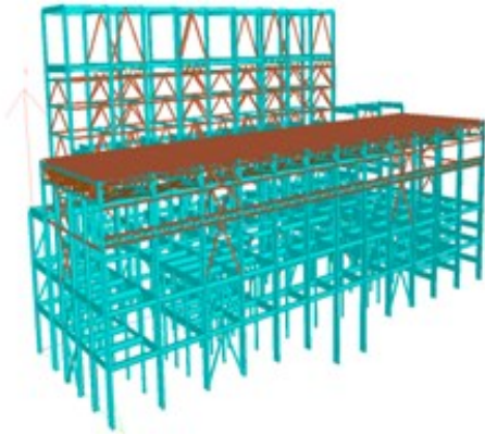
● TG Building
